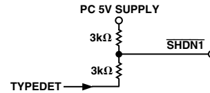
Figure 2. Using \overline{\text{SHDN1}} with TYPEDET Signal
