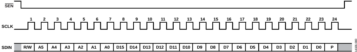
Figure 69. Write Serial Port Timing Diagram
