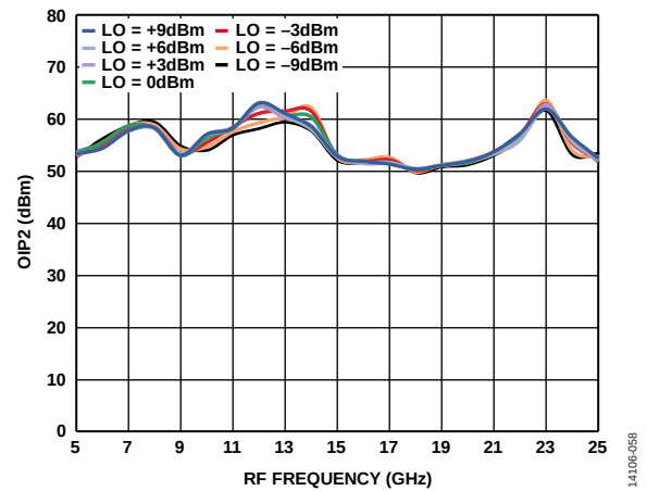
Figure 54. Output Second-Order Intercept (OIP2) vs. RF Frequency ( f_{RF} ) at a 7 dB Gain Setting for Various LO Inputs, IF Amplitude = -15 dBm per Tone
