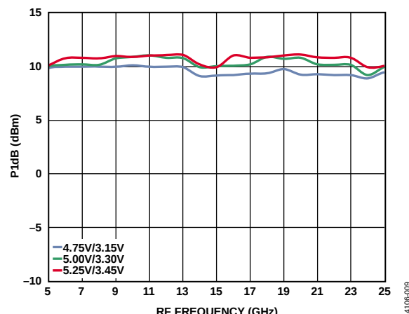
Figure 8. Output 1 dB Compression Point ( P_{1\text{dB}} ) vs. RF Frequency ( f_{\text{RF}} ) at a 10 dB Gain Setting for Various Supply Voltages
