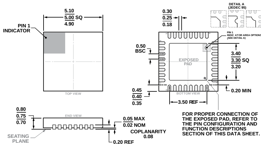
Figure 86. 32-Lead Lead Frame Chip Scale Package [LFCSP] 5 mm × 5 mm Body and 0.75 mm Package Height (CP-32-20)
