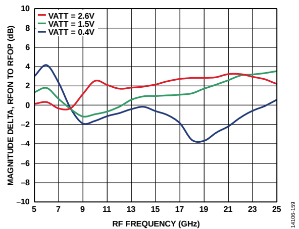
Figure 59. Magnitude Delta, RFON to RFOP vs. RF Frequency ( f_{RF} ) at Three Different Gain Settings
