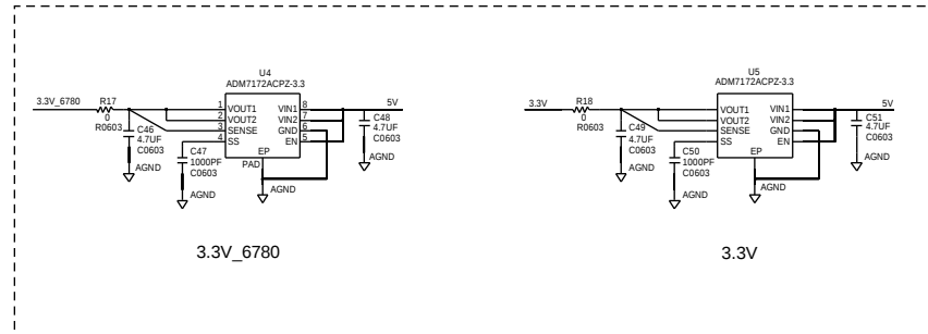
Figure 85. ADRF6780 Evaluation Board Schematic Page 3
