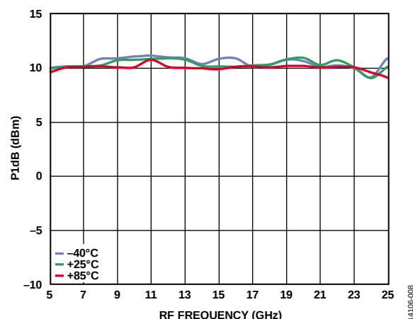
Figure 7. Output 1 dB Compression Point ( P_{1\text{dB}} ) vs. RF Frequency ( f_{\text{RF}} ) at a 10 dB Gain Setting for Various Temperatures
