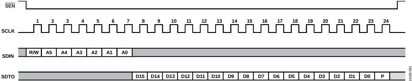
Figure 70. Read Serial Port Timing Diagram
