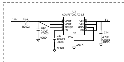
Figure 84. ADRF6780 Evaluation Board Schematic Page 2
