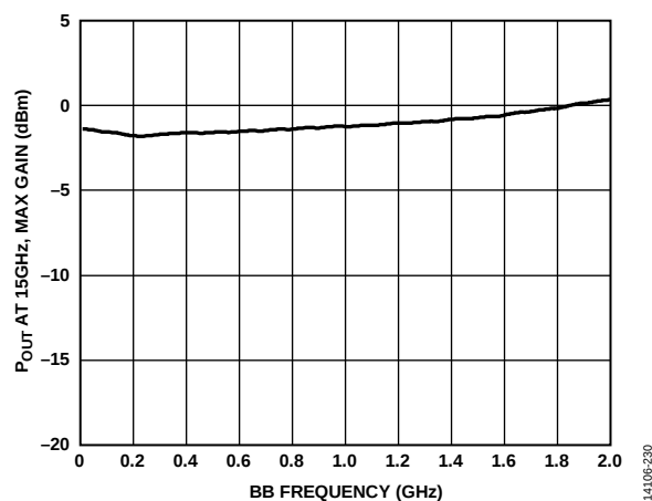
Figure 30. Bandwidth, P_{OUT} at 15 GHz and the Maximum Gain Setting vs. BB Input Frequency
