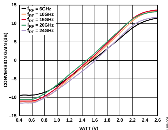
Figure 6. Conversion Gain vs. VATT for Various RF Frequencies ( f_{\text{RF}} )
