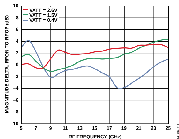
Figure 31. Magnitude Delta, RFON minus RFOP vs. RF Frequency ( f_{RF} ) at Three Different Gain Settings
