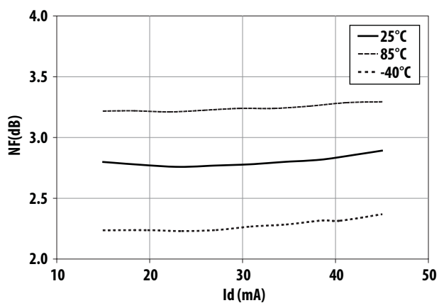
Figure 13. NF vs I_d and Temperature at 900 MHz
