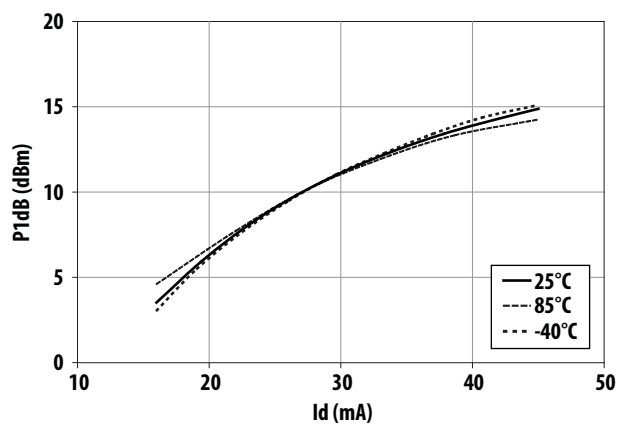
Figure 15. P1dB vs I_d and Temperature at 2 GHz
