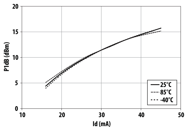
Figure 11. P1dB vs I_d and Temperature at 900 MHz
