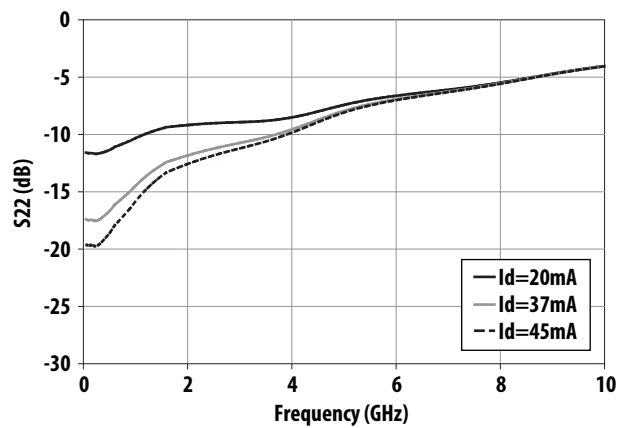
Figure 23. S_{22} vs Frequency and I_d
