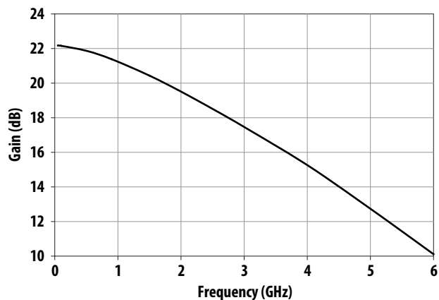
Figure 5. Gain vs Frequency at I_d = 37\text{mA}
