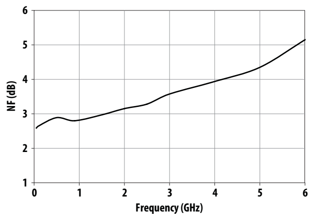
Figure 8. NF vs Frequency at I_d = 37\text{mA}
