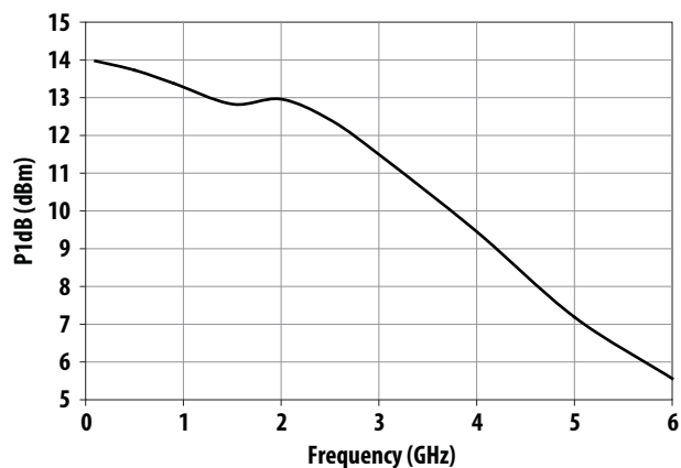
Figure 6. P1dB vs Frequency at I_d = 37\text{mA}
