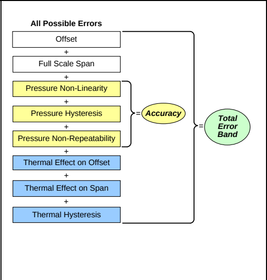
Figure 4. Total Error Band
