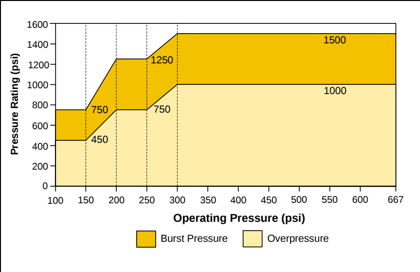
Figure 3. Pressure Rating Curve
