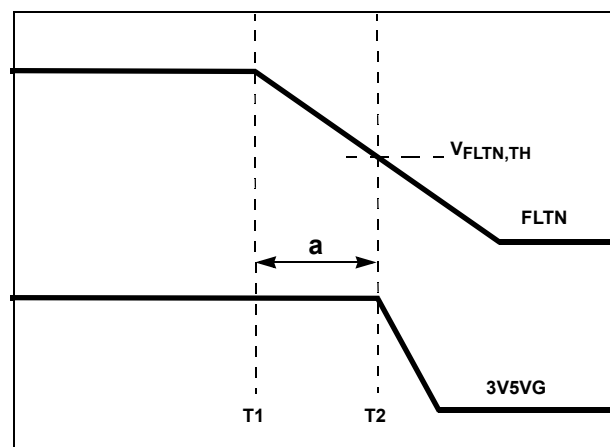
FIGURE 5. TIMING DIAGRAM
