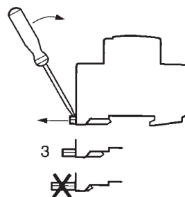
D Insertion when pro M compact cross wiring remains in place
