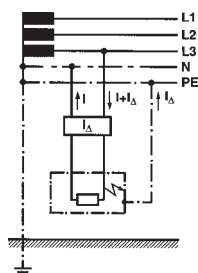
TN-S system (protective multiple earthing) separate neutral and protective conductors throughout the network
