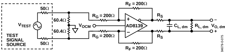
Figure 6. Capacitive Load Test Circuit, G = +1
