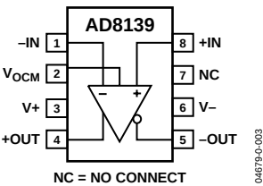
Figure 4. Pin Configuration
