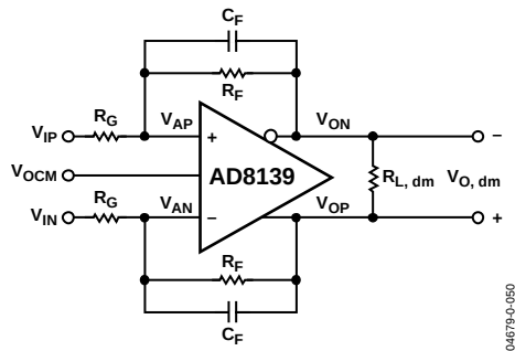
Figure 57. Typical Connection
