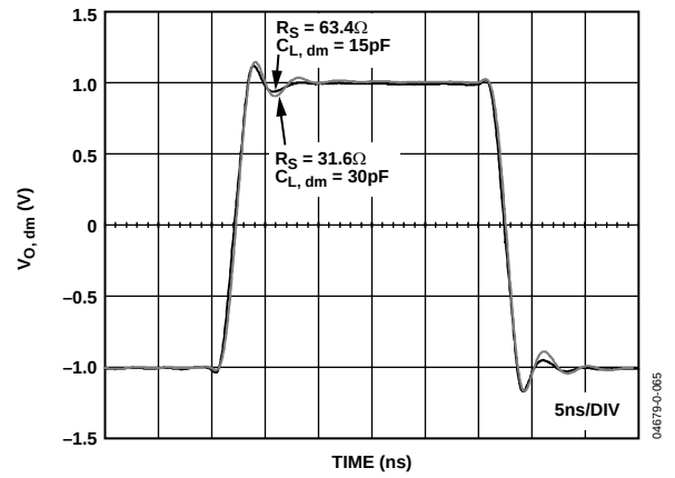
Figure 35. Large Signal Transient Response for Capacitive Loads
