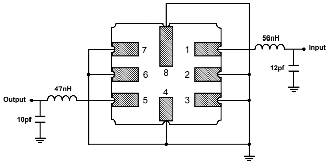
Matching Circuit to 50Ω
