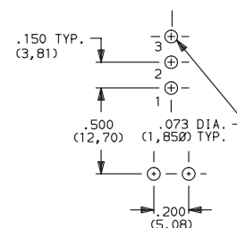
Third Angle Projection
