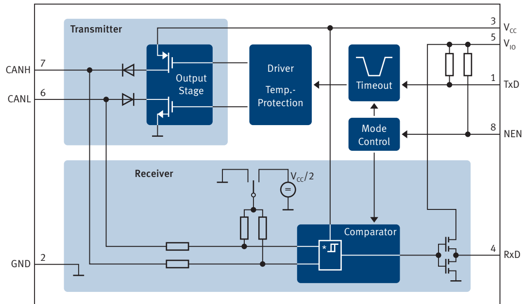
Block Diagram Example High-Speed CAN: TLE7250GVIO
