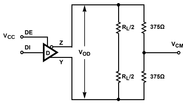
FIGURE 3B. V_{OD} WITH COMMON MODE LOAD
