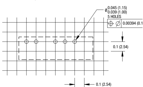
7 Pin SIP Package
