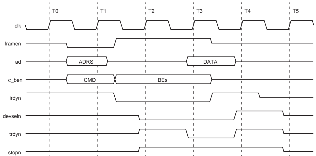
Figure 7. Master Read Single (PCI Bus, 64-Bit)
