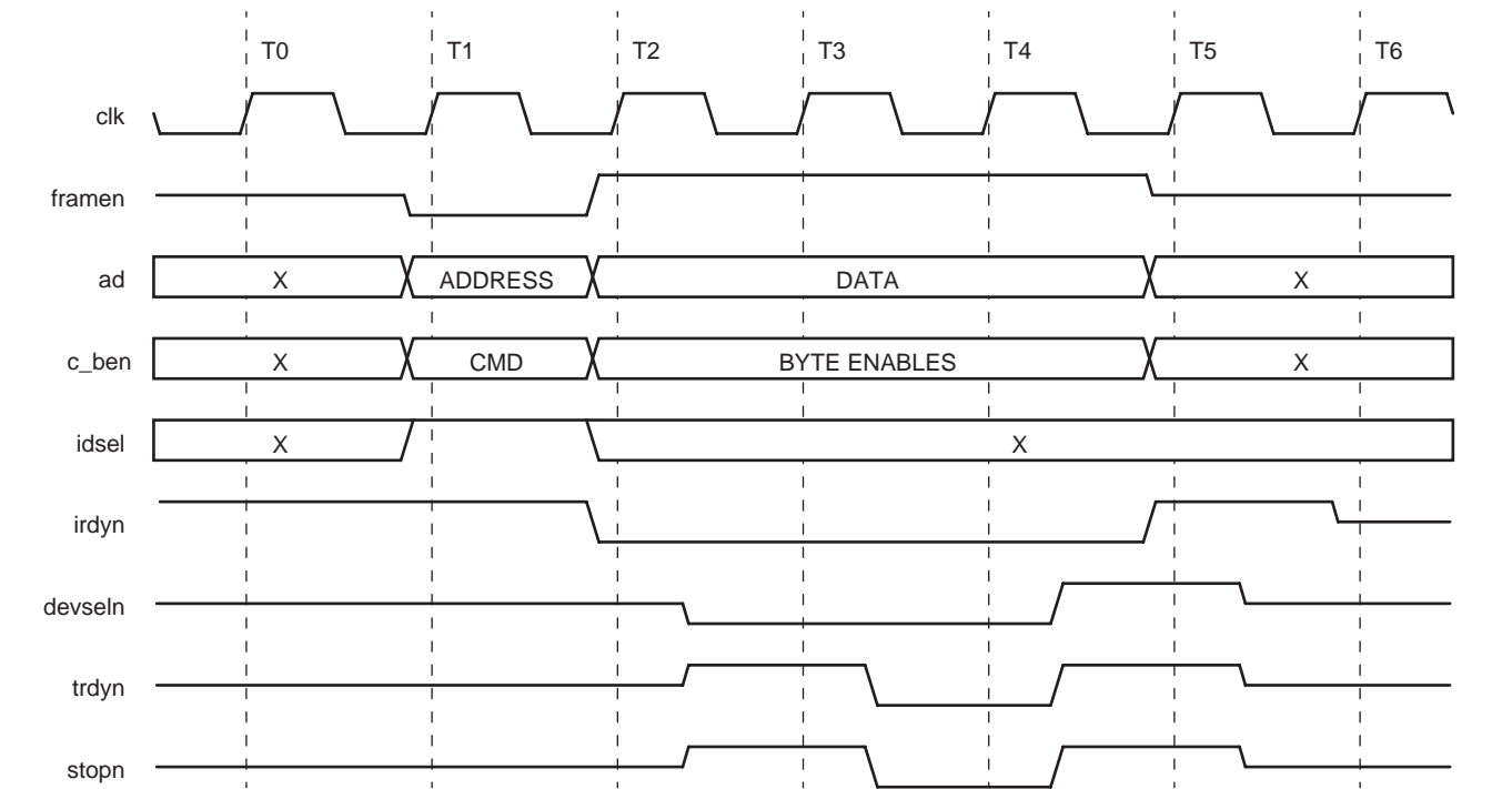
Figure 10. Target Configuration Write (PCI Bus, 64-Bit)
