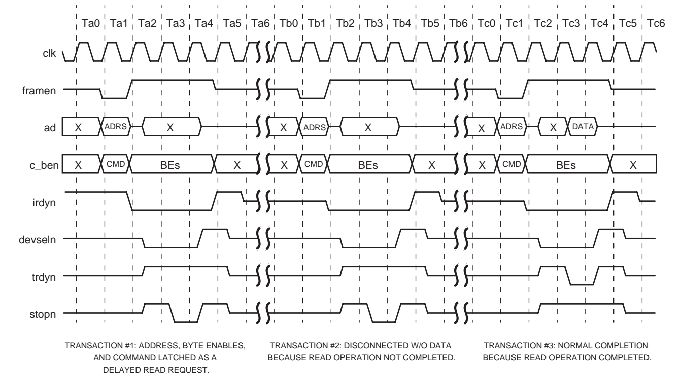
Figure 42. Target Memory Single Read, Delayed (PCI Bus, 64-Bit)
