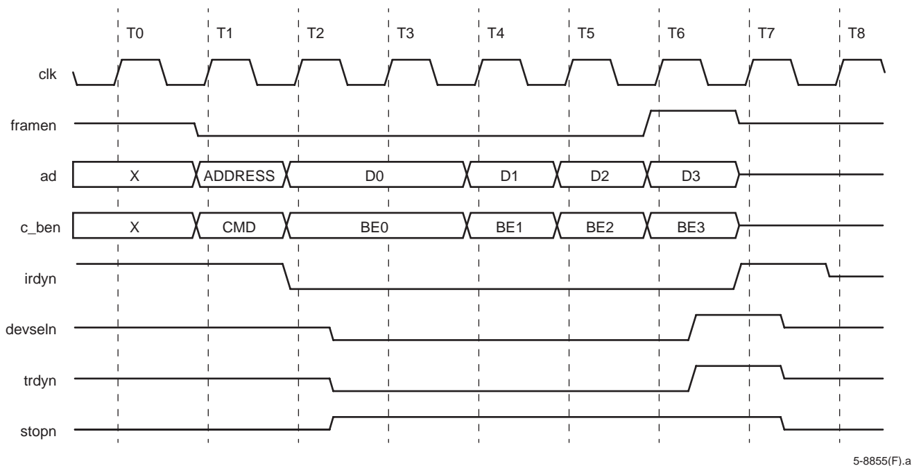
Figure 14. Target Memory Write 32-Byte Burst (PCI Bus, 64-Bit)
