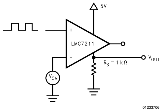
FIGURE 2. Circuit for Measurement of the Shoot-Through Current
