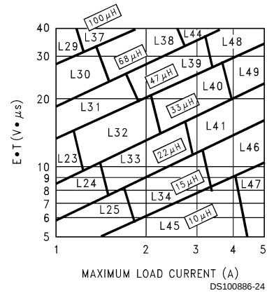
FIGURE 6. LM2678-ADJ
