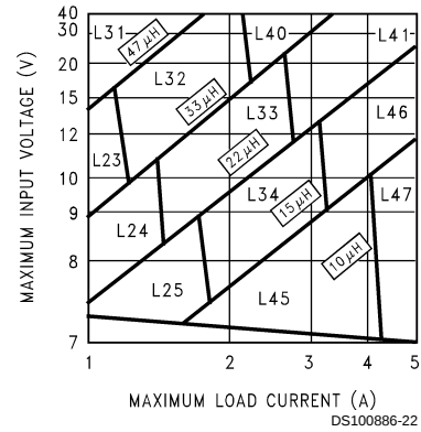
FIGURE 4. LM2678-5.0
