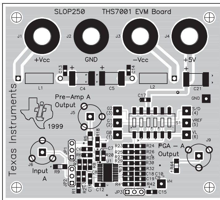
Figure 2–1. THS7001 EVM PC Board: Top Assembly
