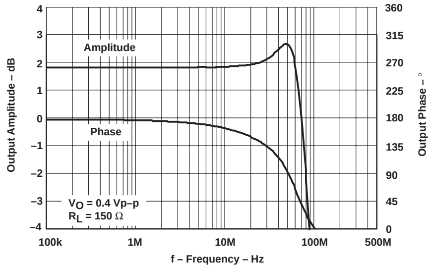
Figure 1–8. THS7001 EVM PGA Response, V_{CC} = \pm 5\text{ V}
