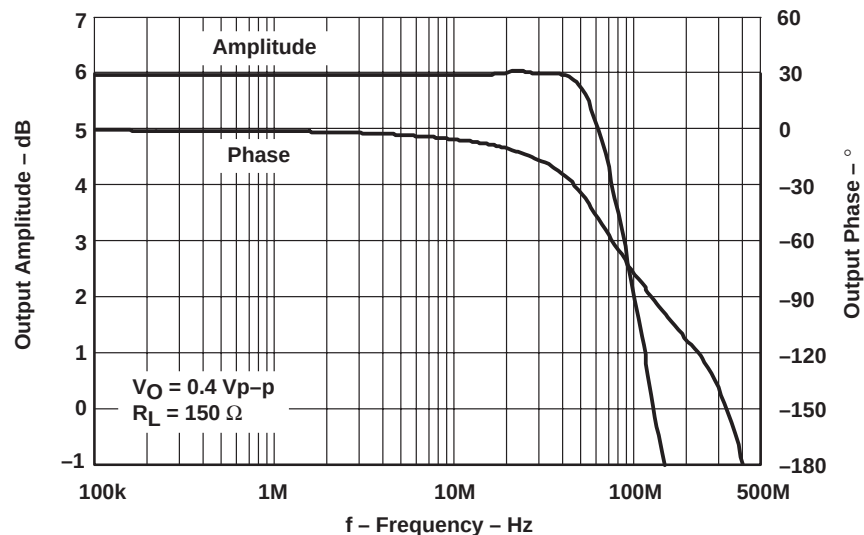
Figure 1–6. THS7001 EVM Preamplifier Response, V_{CC} = \pm 5\text{ V}
