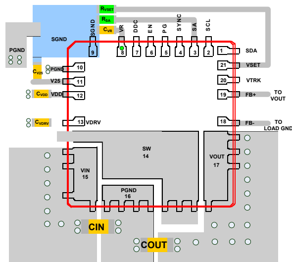
FIGURE 21. RECOMMENDED LAYOUT
