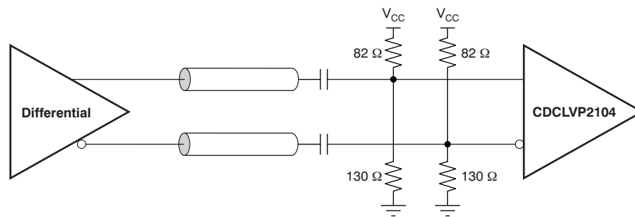
Figure 19. AC-Coupled Differential Inputs to CDCLVP2104 (V CC = 3.3 V)
