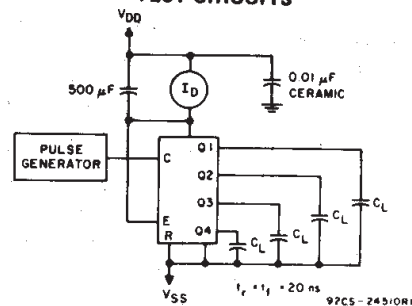
Fig. 10 — Dynamic power dissipation.
