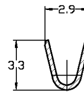
SECT. "B"—"B"
