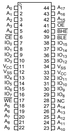
Figure 3. 44-Pin SOJ/TSOP II
