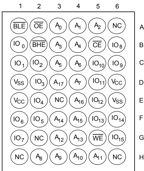
Figure 1. 48-Ball VFBGA (Pinout 1) [2, 3]
