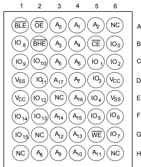
Figure 2. 48-Ball VFBGA (Pinout 2) [2, 3]
