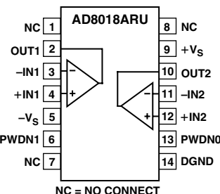
14-Lead TSSOP
