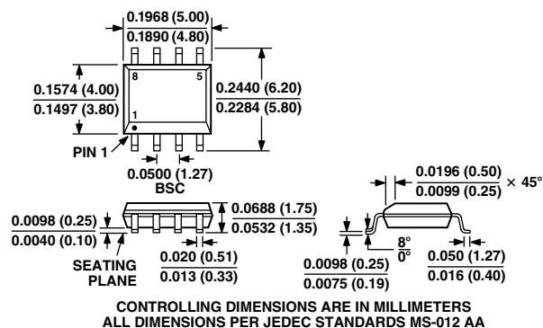
8 Lead SOIC (SO-8)
