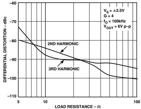
TPC 16. Differential Distortion vs. R_{LOAD}
