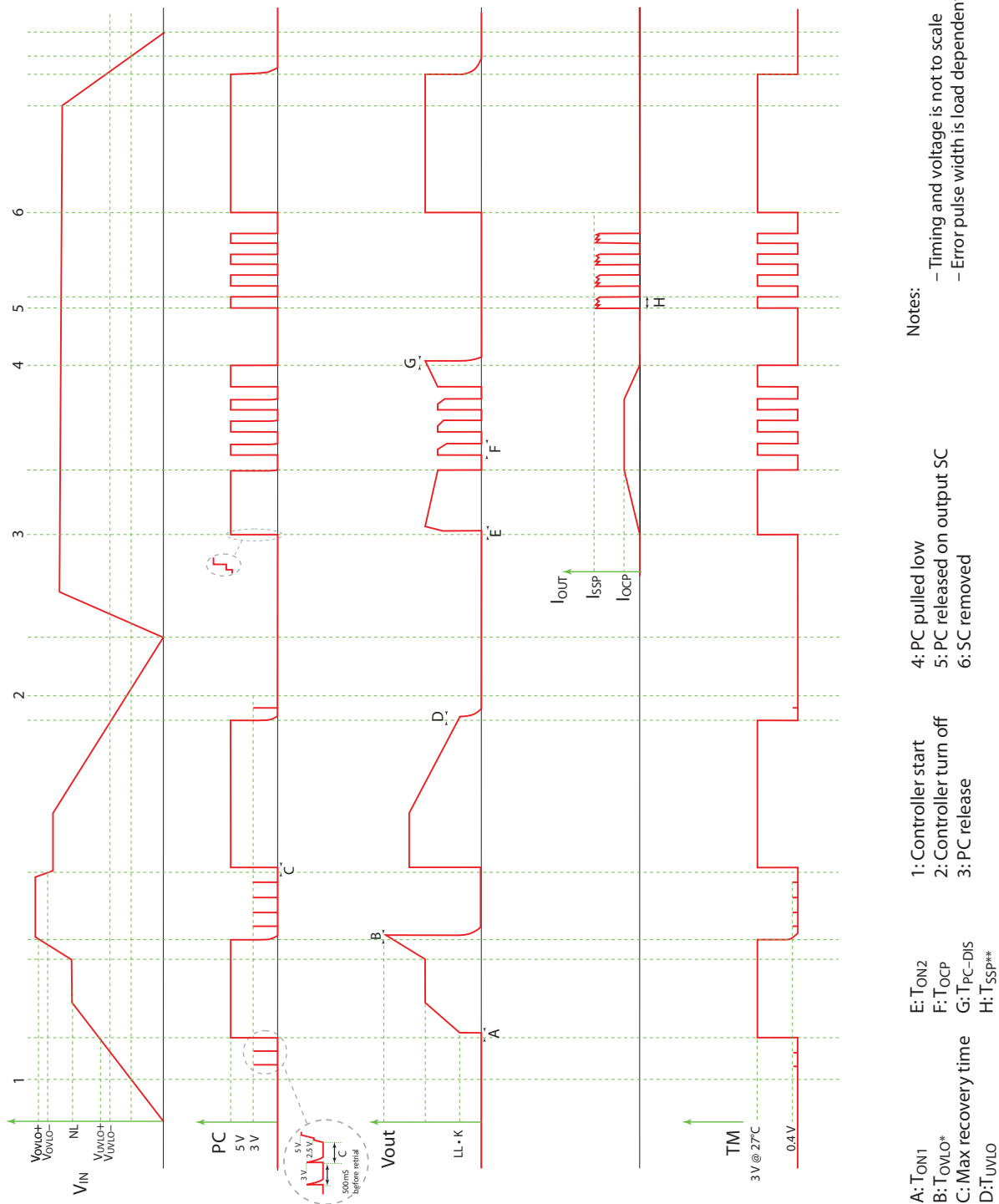
Figure 16 – Timing diagram
