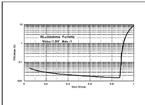
THD + NOISE vs OUTPUT VOLTAGE
