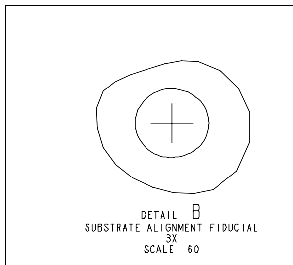
Figure 4. Intel® SCH Package (Solder Resist Opening)
