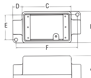
Fig. C Thru-Feed
