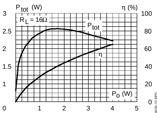
Figure 9 : Power Dissipation and Efficiency versus Output Power
