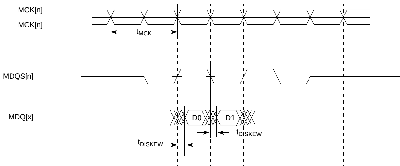
Figure 6. Timing Diagram for t_{\text{DISKEW}}
