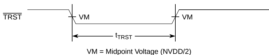
Figure 30. \overline{\text{TRST}} Timing Diagram
