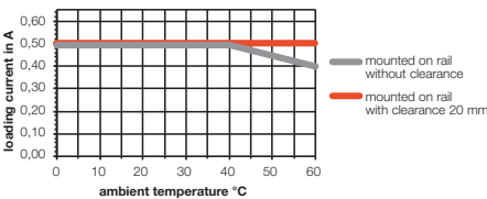
Derating curve MCZ OVP
