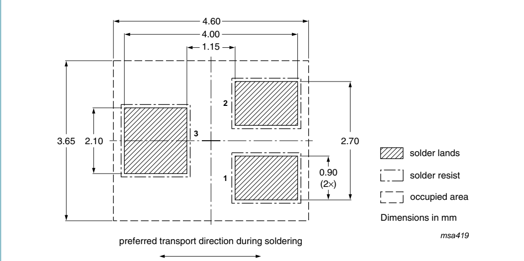
Fig 10. Wave soldering footprint SOT323 (SC-70)
