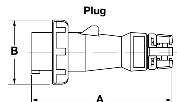
Short Housing Plug
