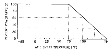
POWER DERATING
