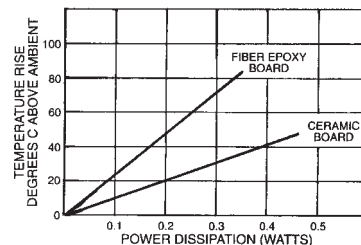
POWER DERATING
