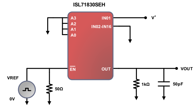
Figure 7. Time to Enable/Disable Output Test Circuit
