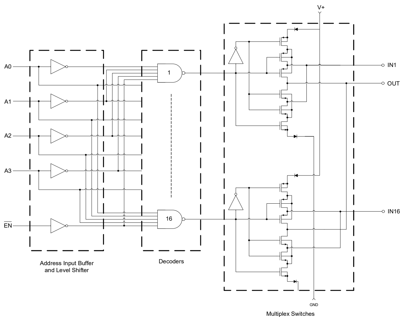
Figure 3. Block Diagram
