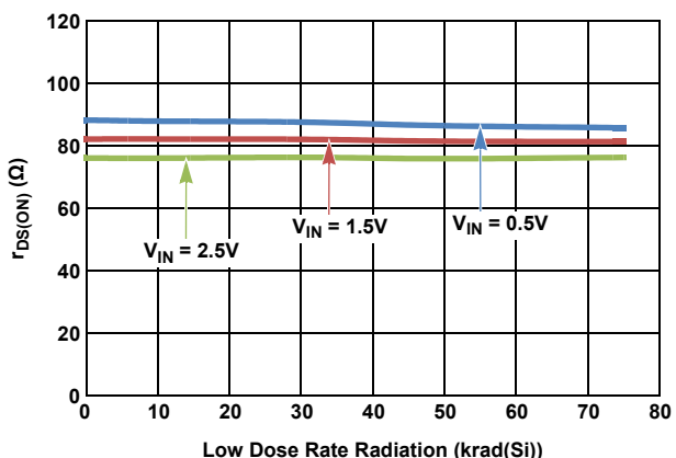
Figure 43. r_{DS(ON)} ( V^+ = 3V ), Biased
