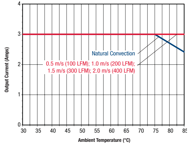
ULE-24/3-D48N-C Temperature Derating Vin 36 (air flow from Pin 1 to Pin 3 on PCB)
