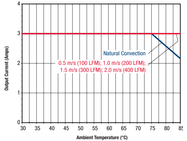
ULE-24/3-D48N-C Temperature Derating Vin 60 (air flow from Pin 1 to Pin 3 on PCB)
