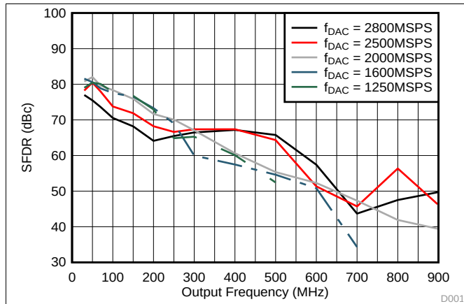
Figure 7. SFDR vs Output Frequency Over f_{DAC}
