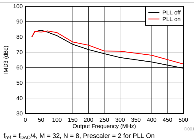
Figure 17. IMD3 vs Output Frequency Over Clocking Options
