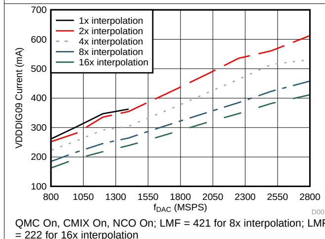
Figure 41. VDDDIG09 Current vs f_{\text{DAC}} Over Interpolation
