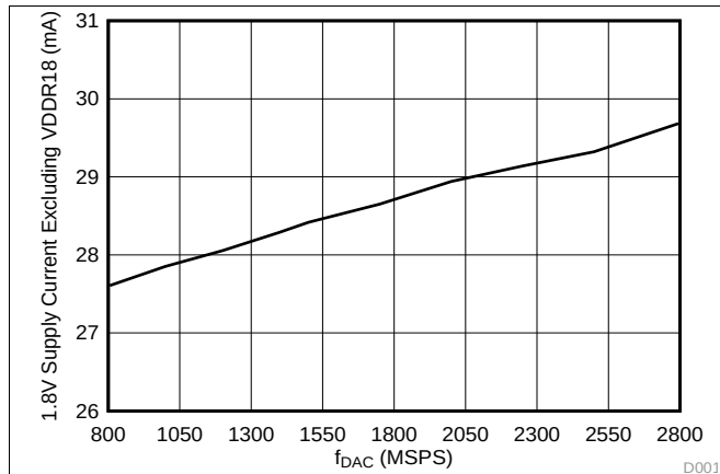
Figure 37. 1.8-V Supply Current Excluding VDDR18 vs f_{\text{DAC}}
