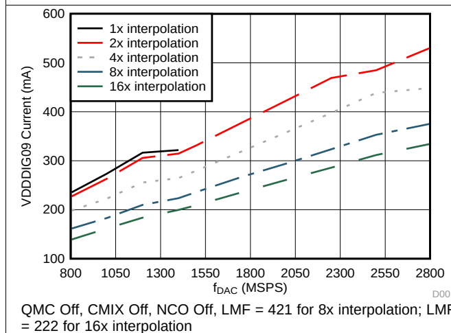
Figure 39. VDDDIG09 Current vs f_{\text{DAC}} Over Interpolation
