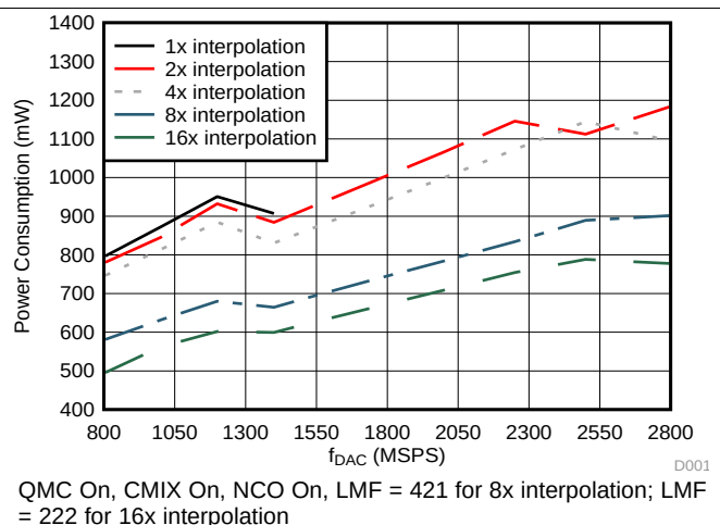
Figure 42. Power Consumption vs f_{\text{DAC}} Over Interpolation
