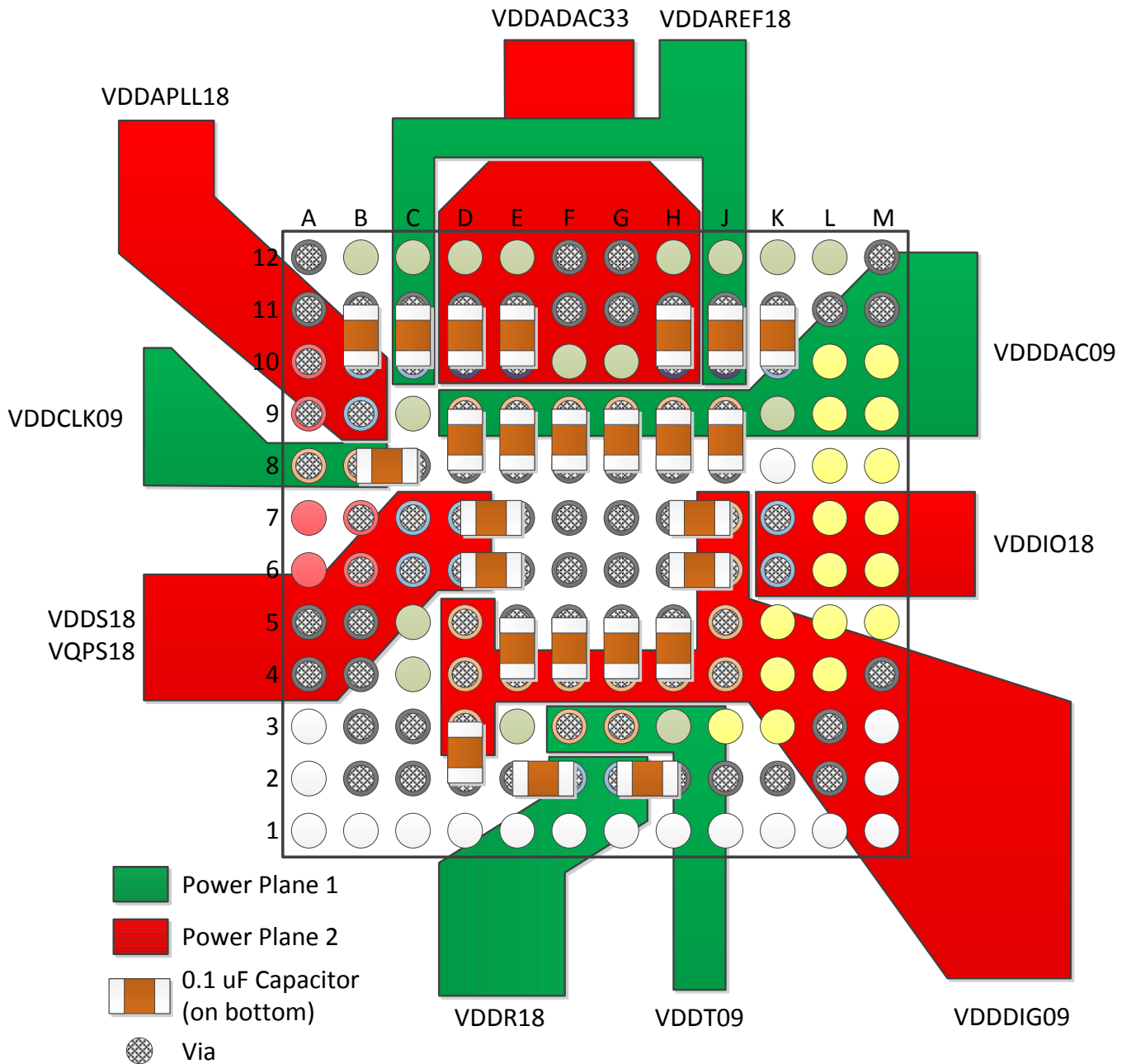
Figure 215. DAC39J82 Layout for Power Supplies
