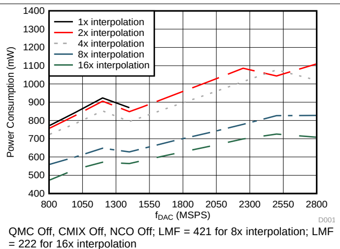
Figure 40. Power Consumption vs f_{\text{DAC}} Over Interpolation
