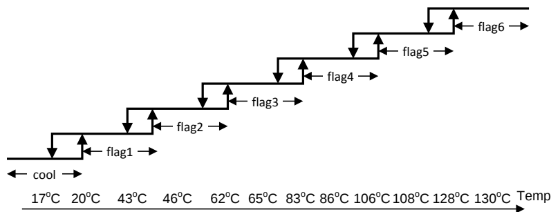
Figure 16. Thermal Shutdown Circuit Features
