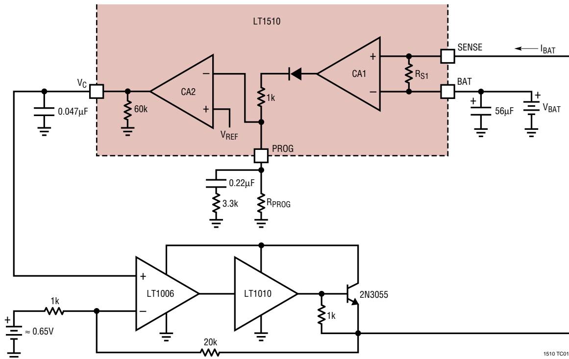
Test Circuit 1
