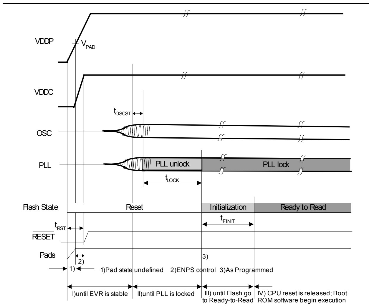
Figure 44 Power-on Reset Timing
