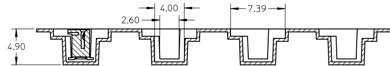
SECTION Z-Z
