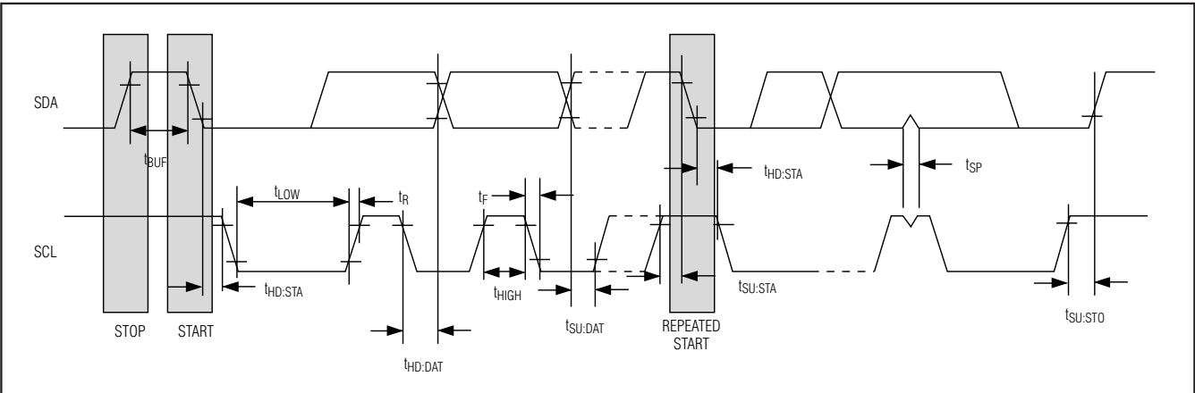
Figure 6. Timing Diagram
