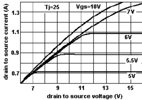
Output Characteristic
