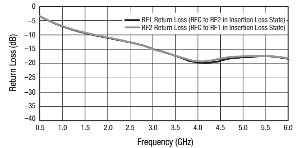
Figure 6. Return Loss vs Frequency (Isolation State)
