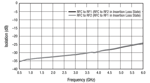
Figure 4. Typical Isolation vs Frequency
