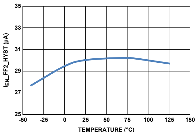
FIGURE 9. EN/VFF2 HYSTERESIS CURRENT vs TEMPERATURE
