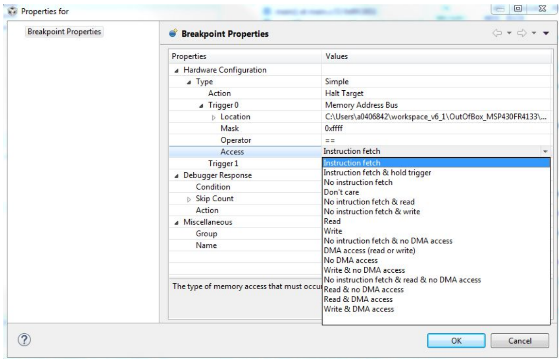
Figure 3-2. Breakpoint Properties
