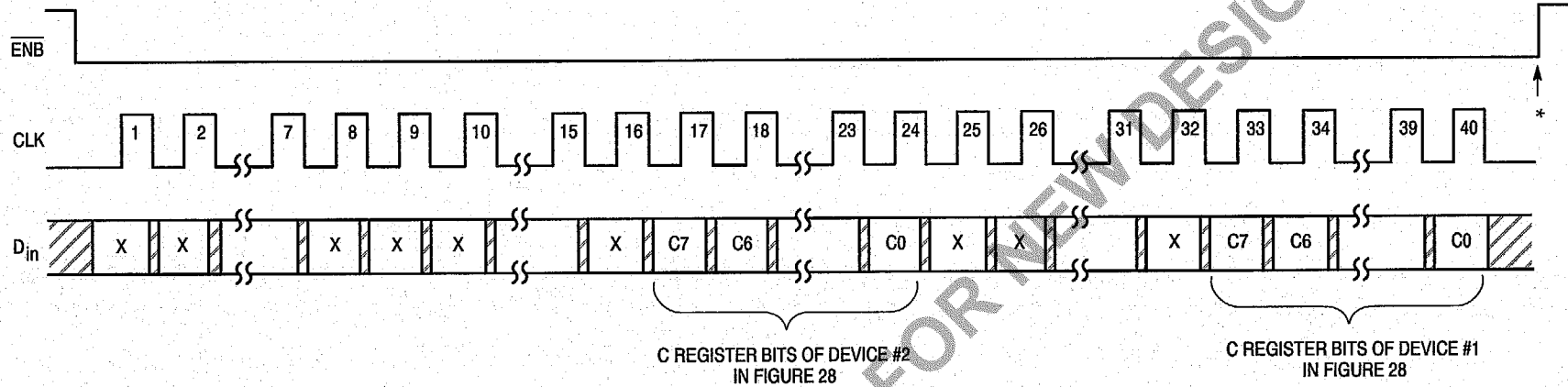
Figure 29. Accessing the C Registers of Two Different Device Types
