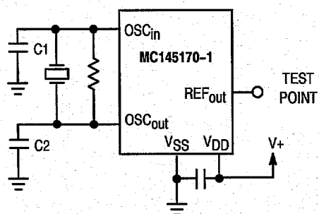
Figure 9. Test Circuit
