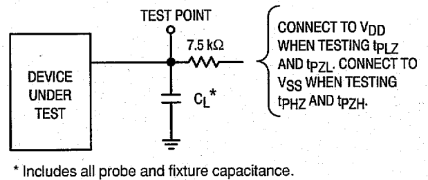
Figure 6. Test Circuit
