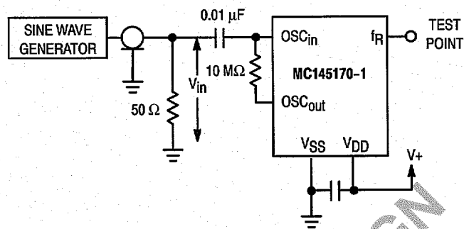
Figure 8. Test Circuit
