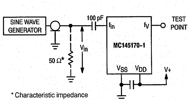
Figure 7. Test Circuit
