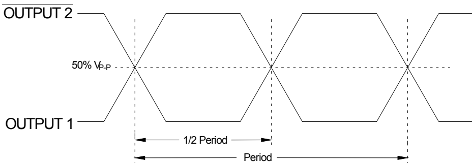
Oscillator Symmetry
