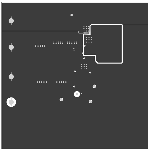
Figure 8. Inner Copper 1
