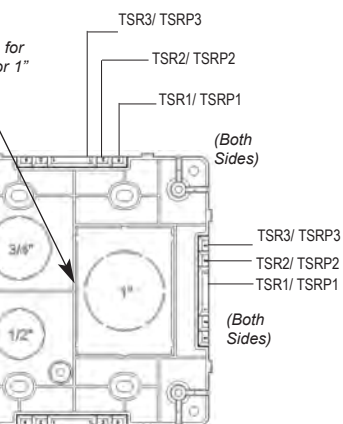
JBD, JBD2 - DUAL GANG
