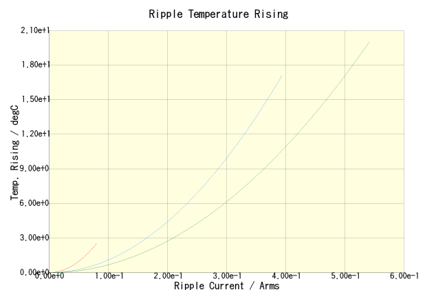
CKCL44X7R1C223M085AA(100kHz) CKCL44X7R1C223M085AA(500kHz) CKCL44X7R1C223M085AA(1MHz)
