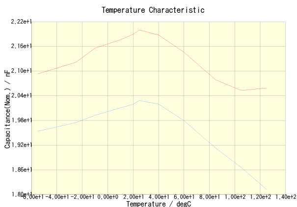
CKCL44X7R1C223M085AA(DC Bias = 0V) CKCL44X7R1C223M085AA(DC Bias = 8V)
