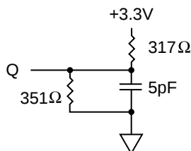
Figure 2 3.3V I/O OUTPUT LOAD EQUIVALENT
